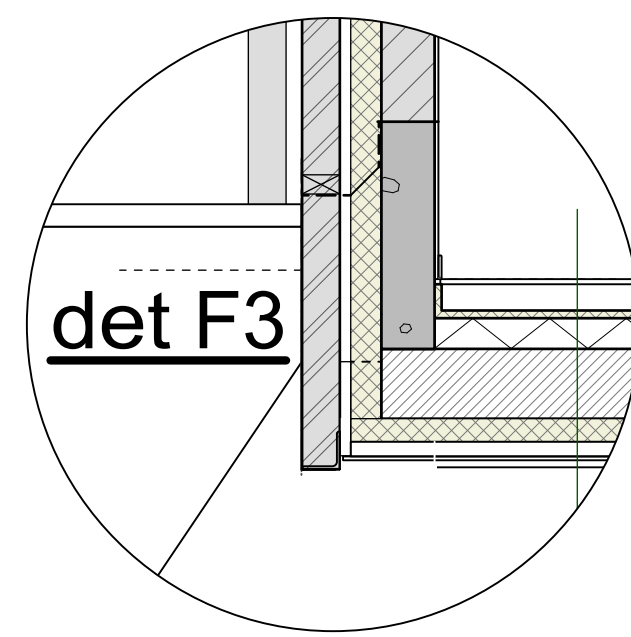
Details snee DD'-schaal 1/20
